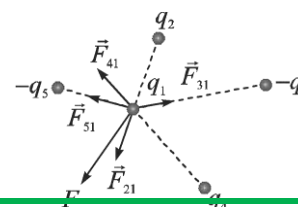
Superposition of electric forces
