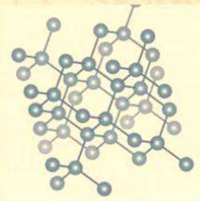
Covalent solid
