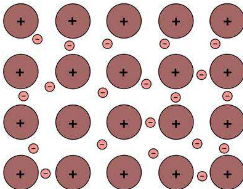
Metallic Solids
