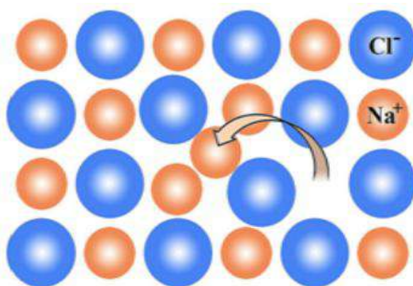
Frenkel defect
