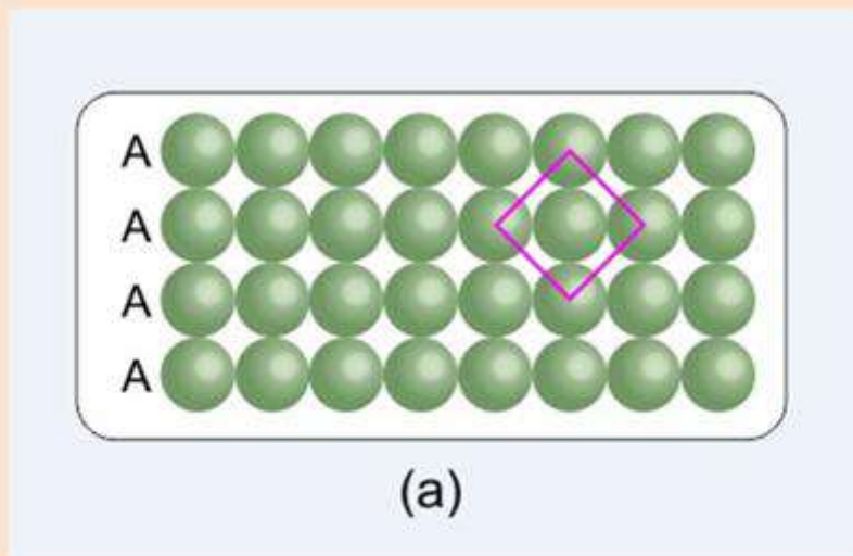
Square close packing
