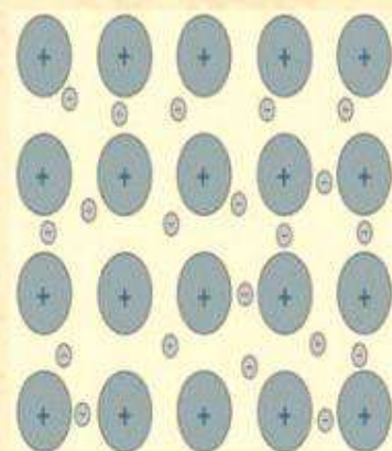
Metallic Solid
