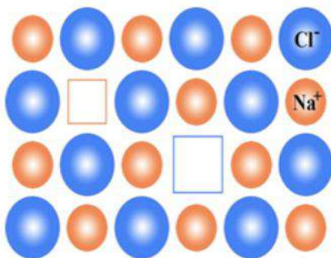
Schottky defect
