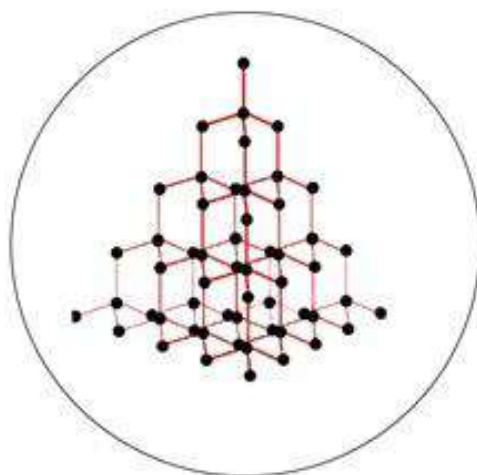
Covalent Solids
