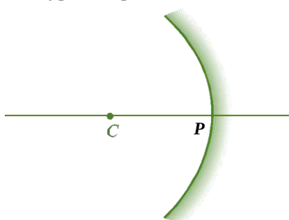
(a) Concave mirror
