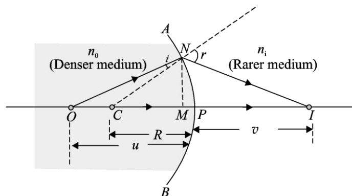
Refraction at a spherical surface – Formation of real image – object
