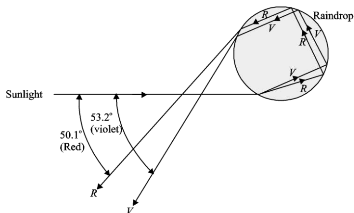
Formation of secondary rainbow
