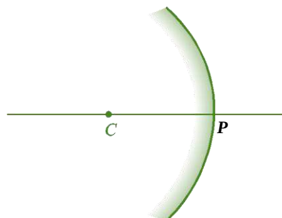
(b) Convex mirror
