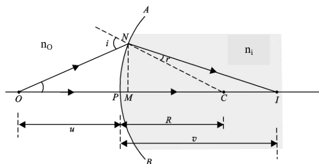
Refraction at spherical surface – Formation of real image - object in a
