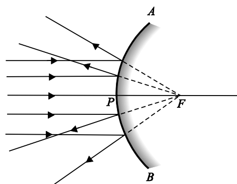
(b) Convex mirror
