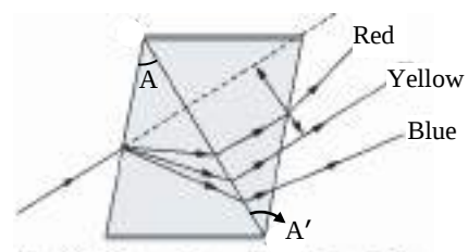
Dispersion without deviation
